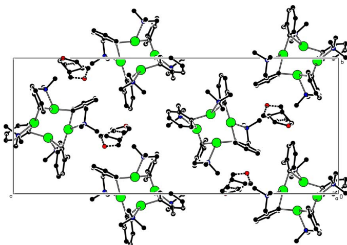
Figure 2 A packing diagram for the P2_12_12_1 polymorph, (I), viewed along the a axis. The THF molecule is disordered over two positions, with relative occupancies of 73% and 27%; dashed lines indicate the minor disorder component.
