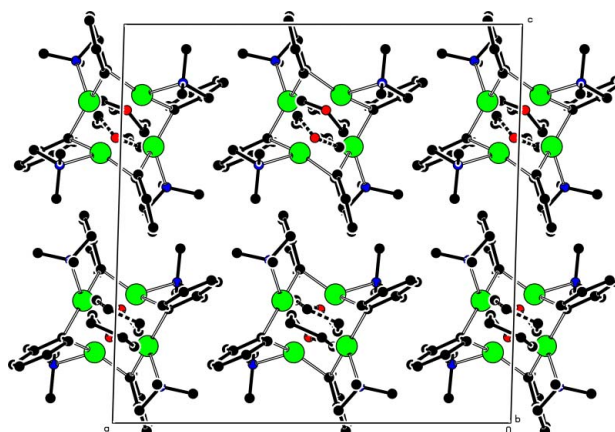
Figure 3 A packing diagram for the C2/c polymorph, (II), viewed along the b axis. The THF molecule is disordered about the twofold axis.
