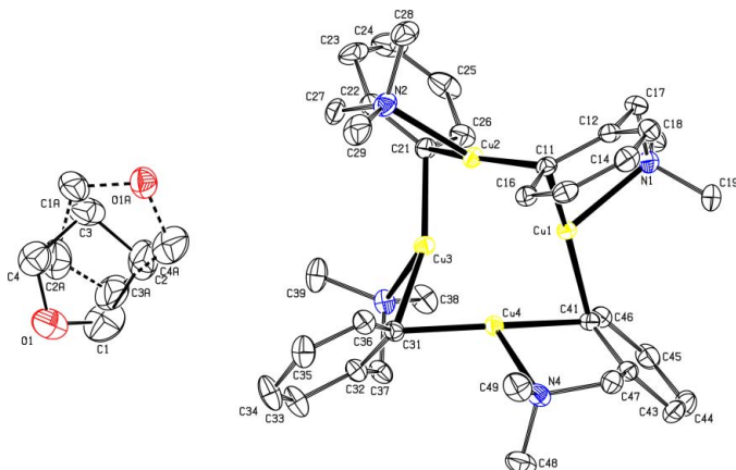
Figure 1 A view of (I), with the atom-numbering scheme. Displacement ellipsoids are drawn at the 50% probability level. H atoms have been omitted for clarity. Both disorder components are shown.
